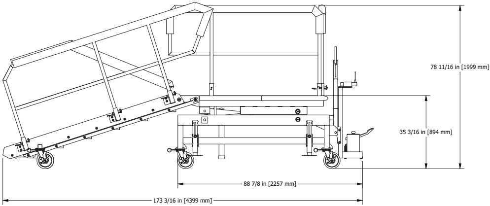
COLLAPSED POSITION
