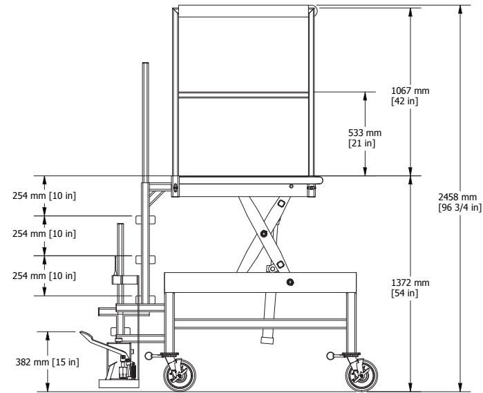
EXTENDED POSITION
