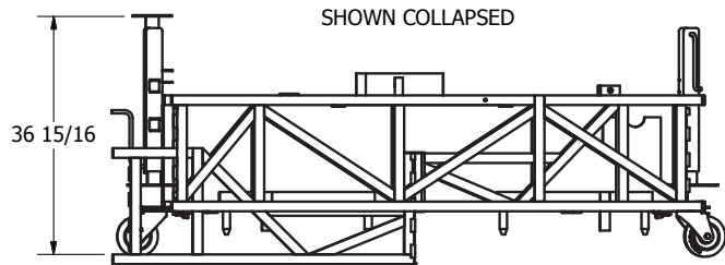
DOLLY DETAILS
