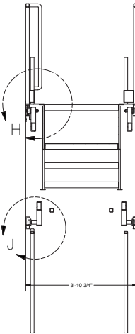
SECTION F-F SCALE 1 / 20
