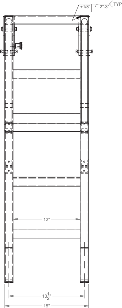
STAND DETAILS
