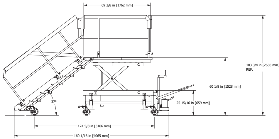
EXTENDED POSITION
