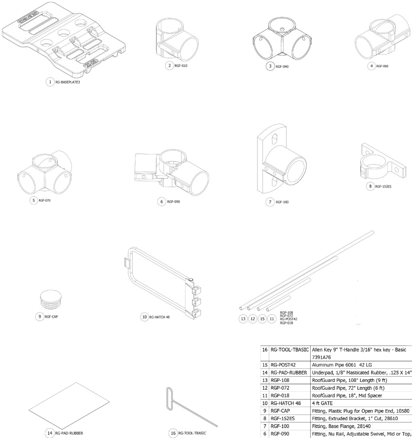
Figure 1 - Component Identification
