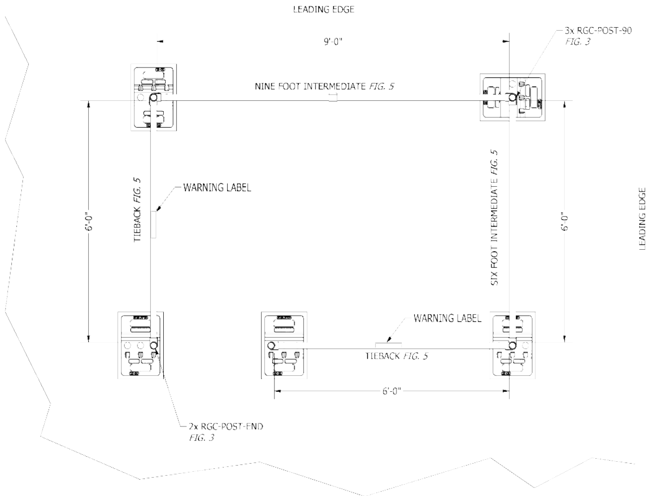
Figure 2 - Typical Layout
