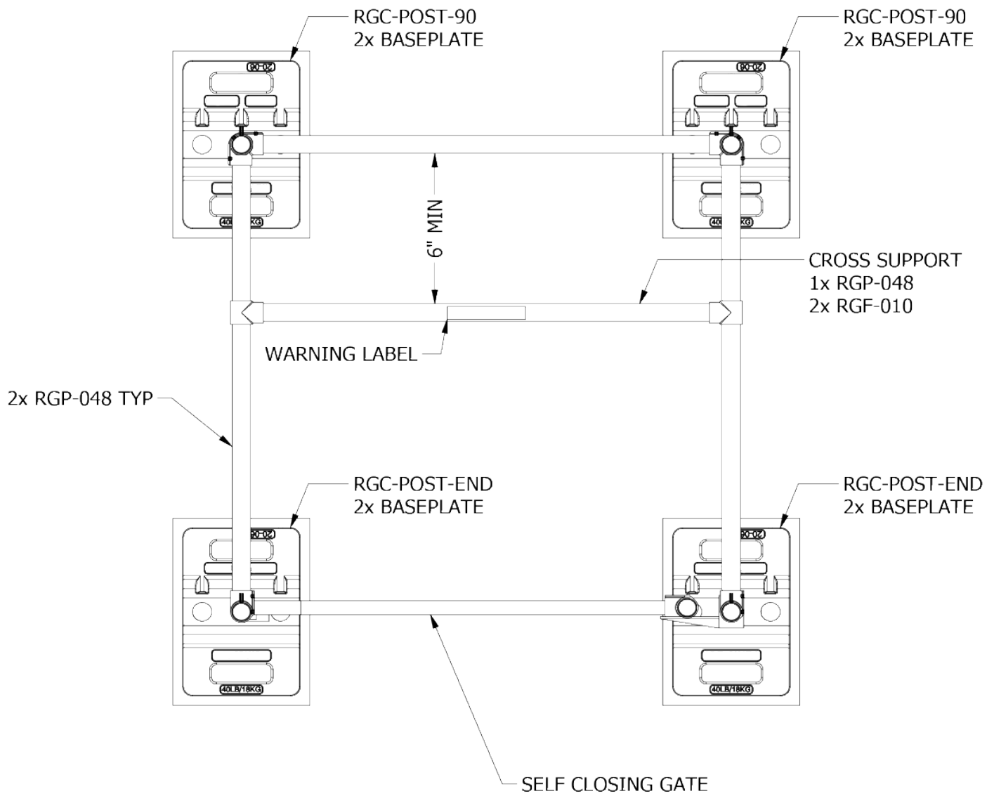
Figure 7 - Hatch Rails
