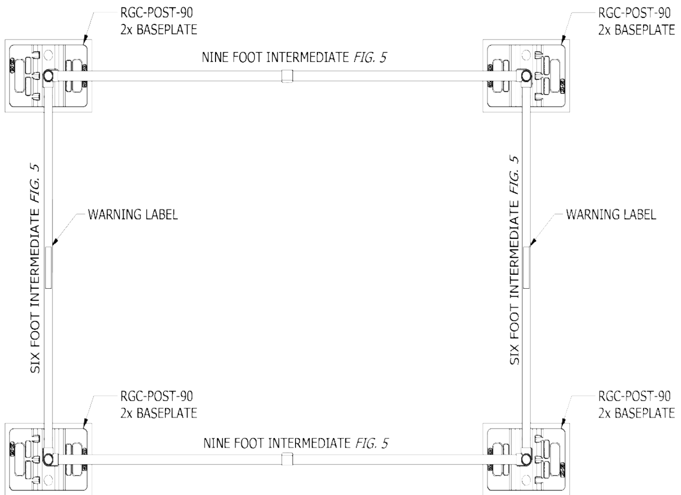
Figure 6 - Skylight Rails
