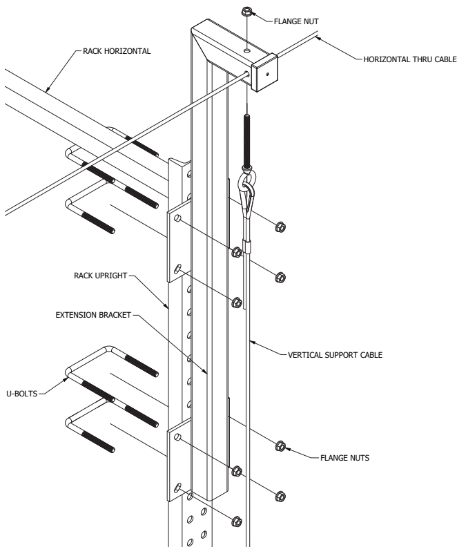
Figure 5 - Extension Bracket
